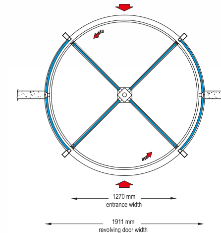
REV190 is a high-security, fully automatic 4-leaf revolving door with a wide range of security options.
